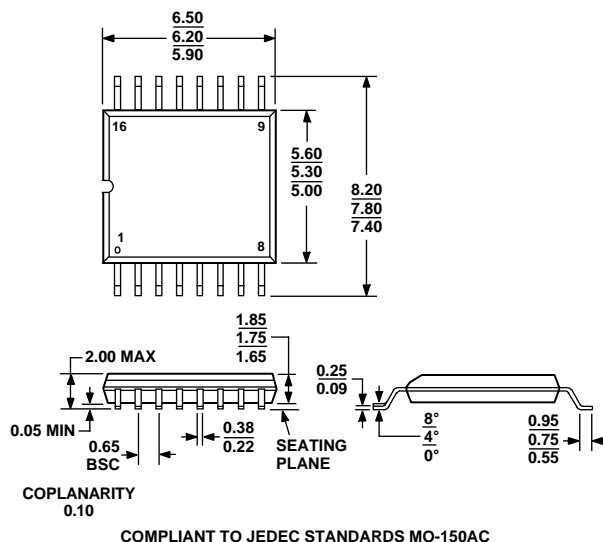
Figure 17 16-Lead Shrink Small Outline Package [SSOP] (RS-16)
