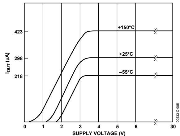
Figure 5. V-I Plot
