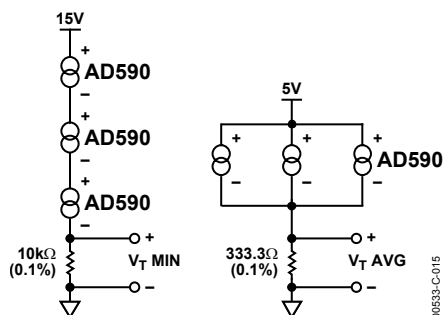
Connecting several AD590 units in series as shown in Figure 15 allows the minimum of all the sensed temperatures to be indicated. In contrast, using the sensors in parallel yields the average of the sensed temperatures.
