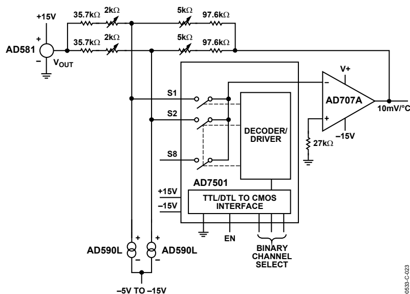
Figure 23. 8-Channel Multiplexer
