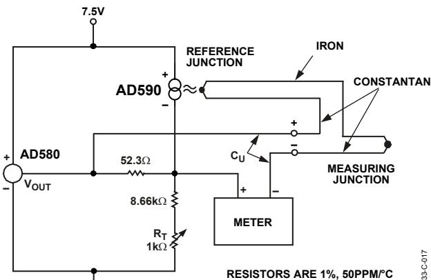
Figure 17 is an example of a cold junction compensation circuit for a Type J thermocouple using the AD590 to monitor the reference junction temperature. This circuit replaces an ice-bath as the thermocouple reference for ambient temperatures between 15°C and 35°C. The circuit is calibrated by adjusting R_T for a proper meter reading with the measuring junction at a known reference temperature and the circuit near 25°C. Using components with the TCs as specified in Figure 17, compensation accuracy is within \pm 0.5^\circ\text{C} for circuit temperatures between 15°C and 35°C. Other thermocouple types can be accommodated with different resistor values. Note that the TCs of the voltage reference and the resistors are the primary contributors to error.
