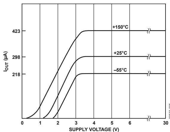
Figure 7. V-I Plot
