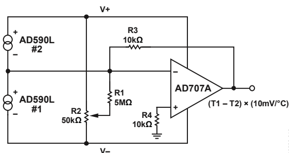
Figure 18. Differential Measurements
