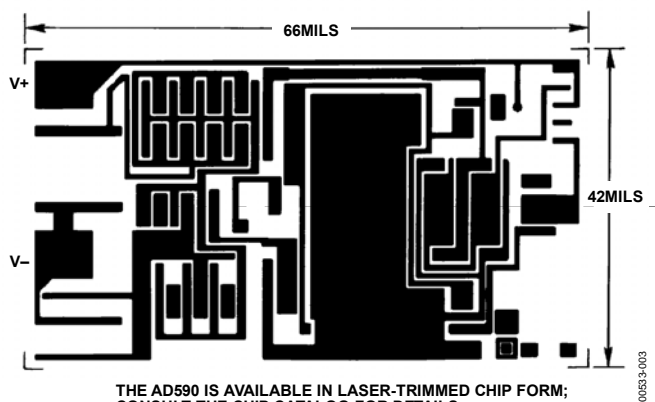
Figure 5. Metallization Diagram
