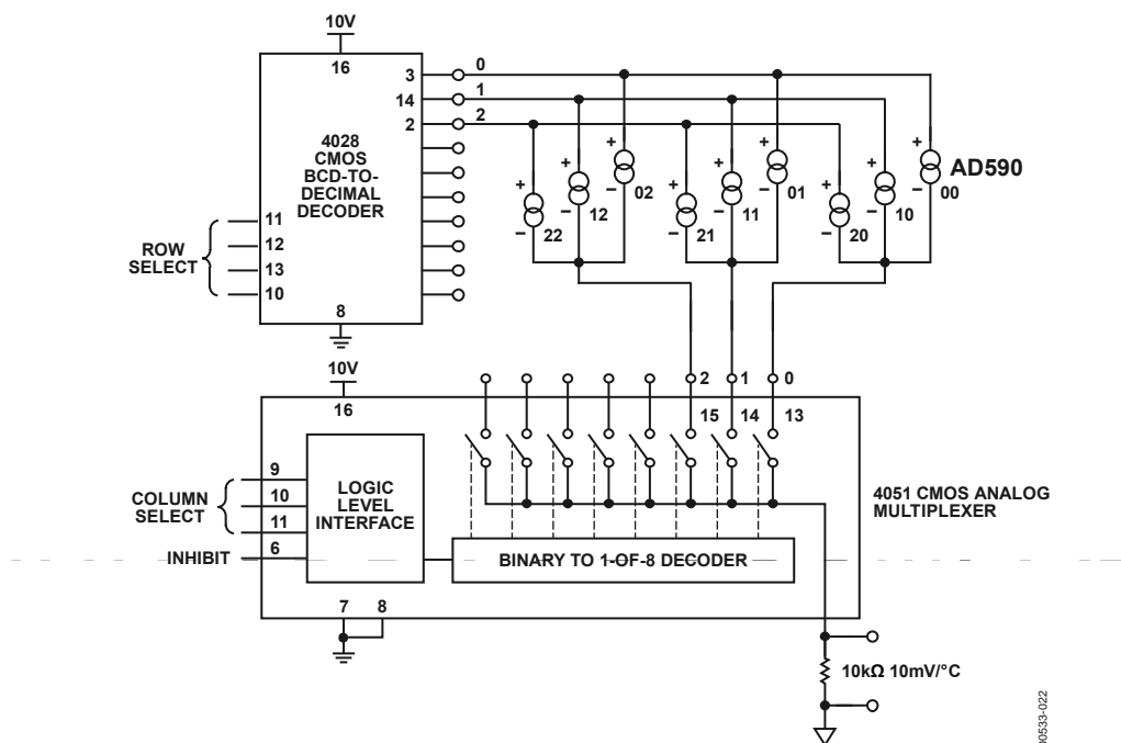
Figure 24. Matrix Multiplexer
