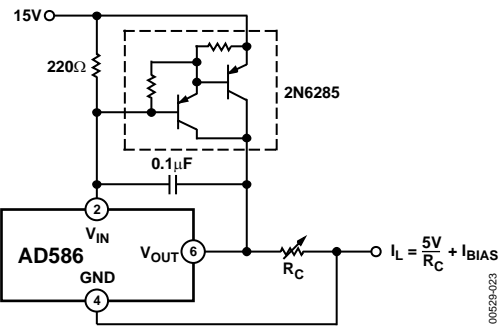
Figure 24. Precision High Current Current Source
