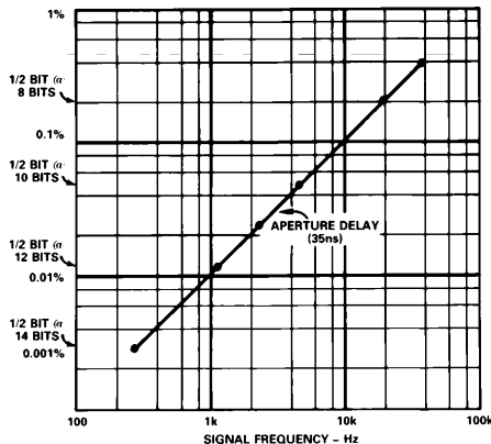
Figure 10. Aperture Delay Error vs. Frequency
