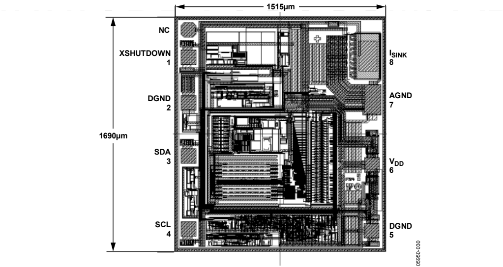
Figure 4. Metallization Photo Dimensions shown in microns (µm)
