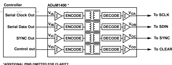
Figure 16. Isolated Interface
