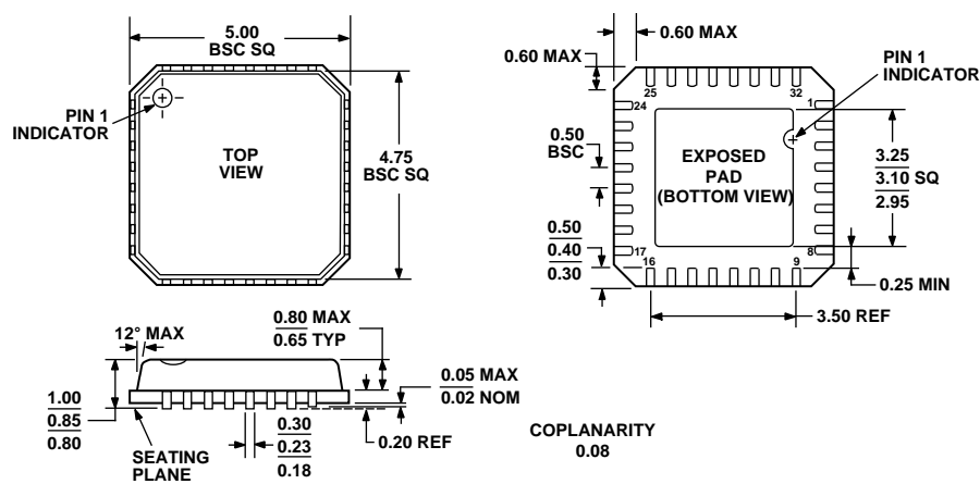
Figure 17. 32-Lead Lead Frame Chip Scale Package (CP-32-2) Dimensions shown in millimeters
