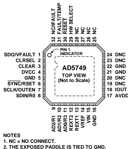
Figure 4. Pin Configuration
