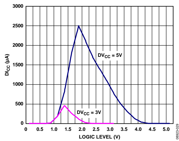
Figure 29. D_{ICC} vs. Logic Input Voltage
