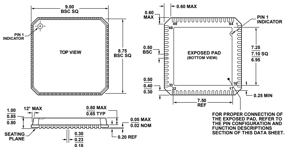
Figure 65. 64-Lead Lead Frame Chip Scale Package [LFCSP_VQ]
