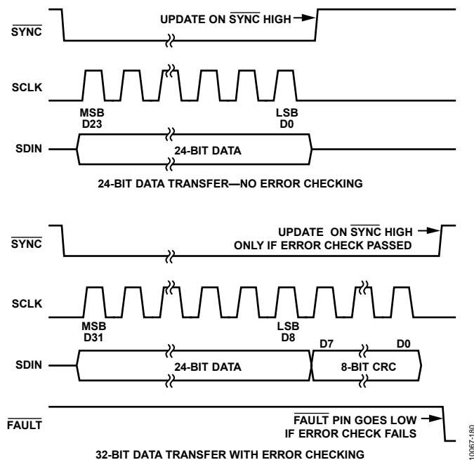
Figure 53. PEC Timing
