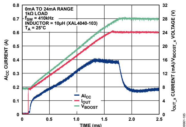
Figure 80. AI_{CC} Current vs. Time for 24 mA Step Through 1 k \Omega Load with External 51 k \Omega Compensation Resistor
