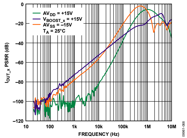
Figure 52. I_{OUT,x} PSRR vs. Frequency
