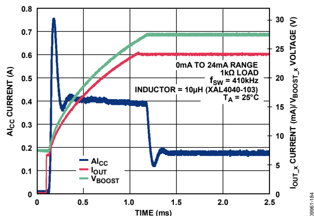
Figure 79. AI_{CC} Current vs. Time for 24 mA Step Through 1 kΩ Load with Internal Compensation Resistor
