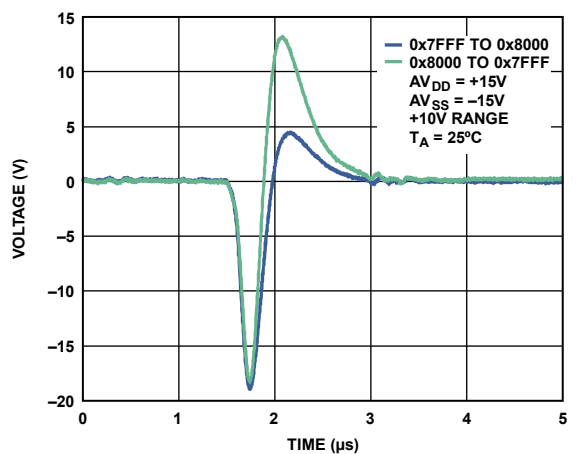
Figure 25. Digital-to-Analog Glitch
