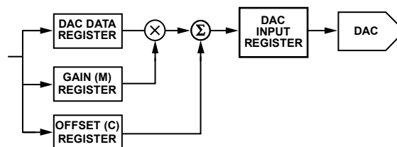
Figure 75. Digital Offset and Gain Control
