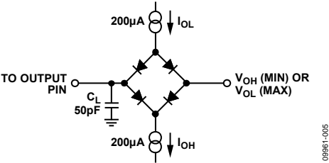
Figure 6. Load Circuit for SDO Timing Diagrams
