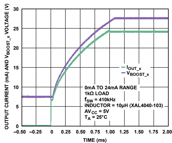
Figure 47. Output Current and V_{BOOST\_x} Settling Time with DC-to-DC Converter (See Figure 77)
