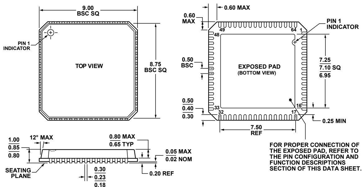
Figure 86. 64-Lead Lead Frame Chip Scale Package [LFCSP_VQ] 9 mm × 9 mm Body, Very Thin Quad (CP-64-3)
