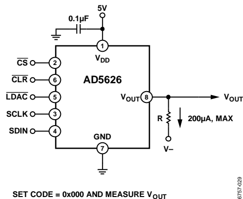
Figure 29. Measuring Zero-Scale or Offset Error
