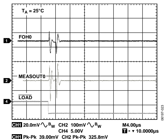
Figure 28. AC Crosstalk, FVMI Mode, PMU 0, Full-Scale Transition on One CPH DAC, MI Gain = 10, MEASOUTx Gain = 1, \pm 2 mA Range, C_{LOAD} = 200 pF
