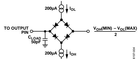
Figure 4. Load Circuit for SDO, \overline{\text{BUSY}} Timing Diagram
