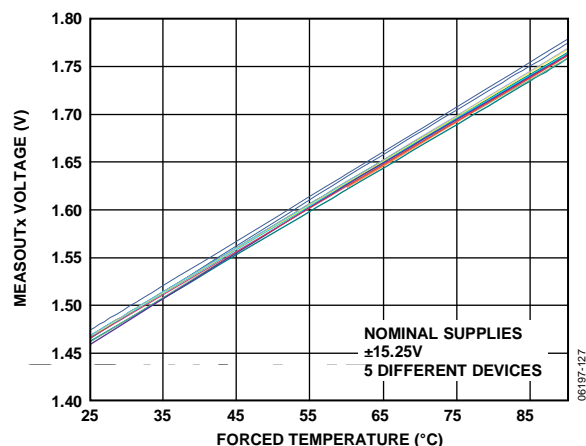
Figure 32. Temperature Sensor Voltage on MEASOUTx vs. Forced Temperature
