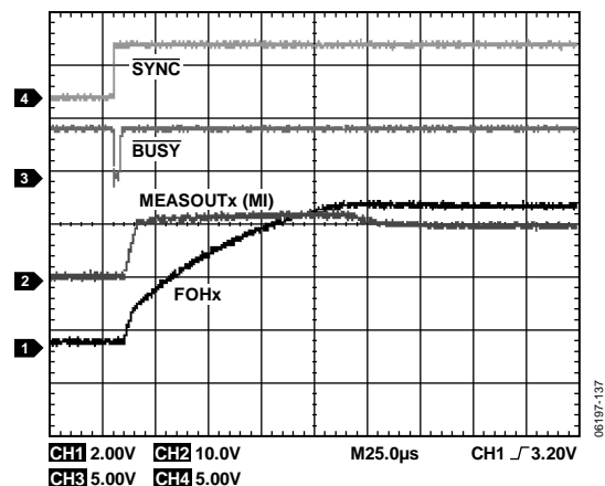
Figure 42. FV Settling, 0 V to 5 V, \pm 20 \mu A Range, C_{LOAD} = 220 pF, CCOMP_x = 100 pF, R_{LOAD} = 270 k \Omega
