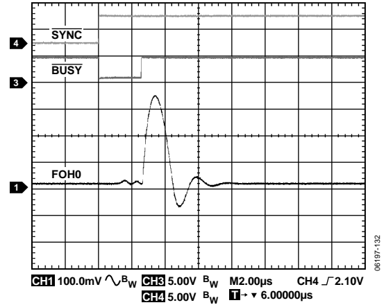
Figure 37. Range Change, PMU 0, \pm 20 \mu\text{A} to \pm 2 \text{ mA} , C_{\text{LOAD}} = 1 \text{ nF} , R_{\text{LOAD}} = 150 \text{ k}\Omega , FV = 3 \text{ V}
