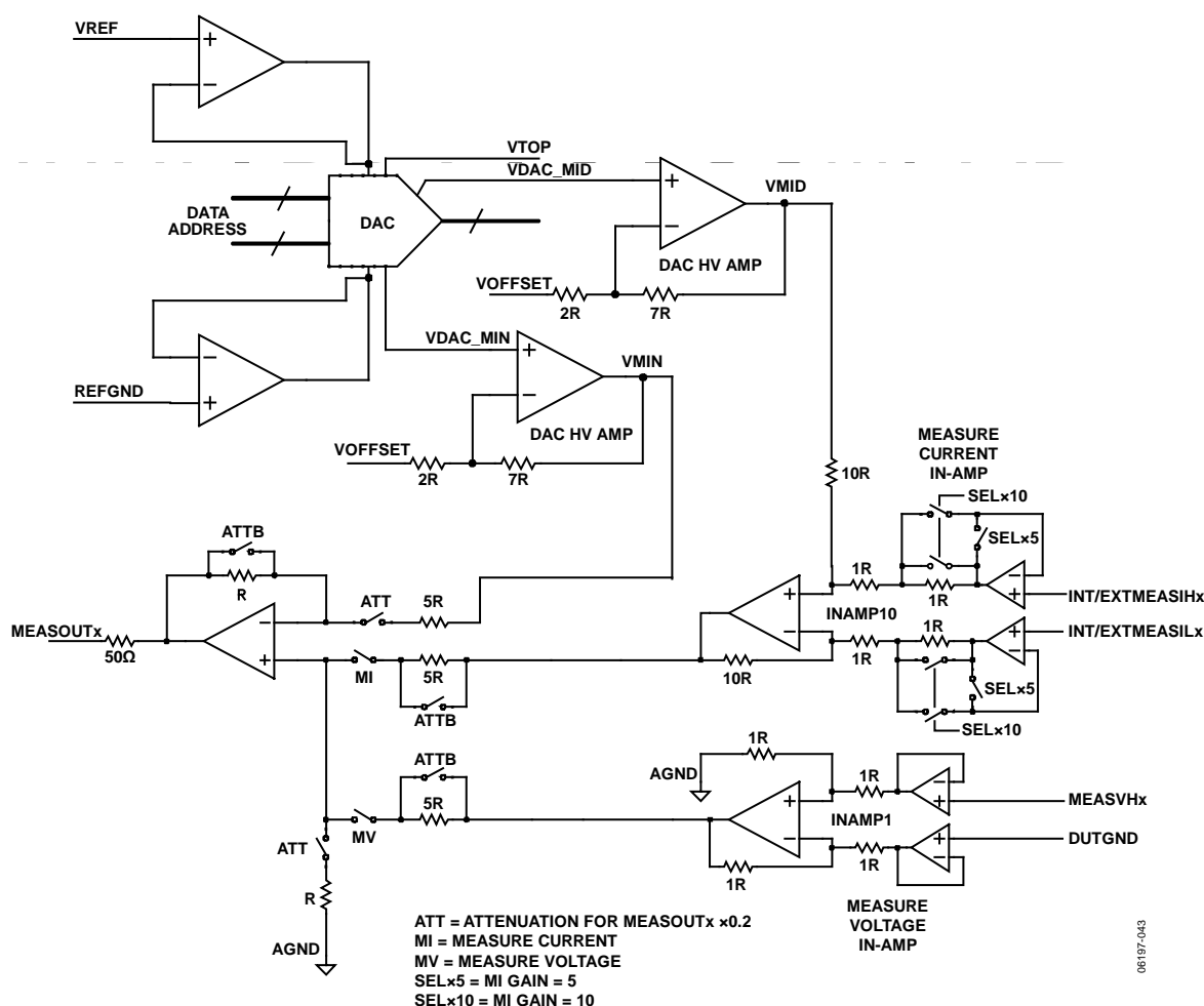
Figure 45. Measure Block and VMID Influence
