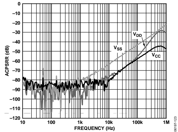
Figure 26. APCSR at MEASOUTx in Measure Current Mode vs. Frequency (MI Gain = 5, Measout Gain = 0.2)
