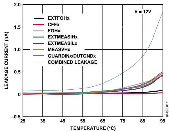
Figure 15. Leakage Current vs. Temperature (Stress Voltage = 12 V)
