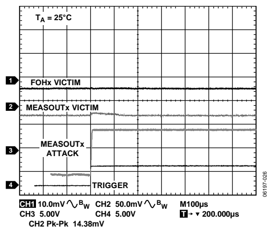
Figure 31. Shorted DUT AC Crosstalk, Victim PMU in FVMI Mode ( \pm 200 \mu A Range)
