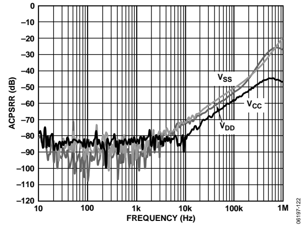
Figure 25. APCSR at MEASOUTx in Measure Current Mode vs. Frequency (MI Gain = 10, Measout Gain = 0.2)
