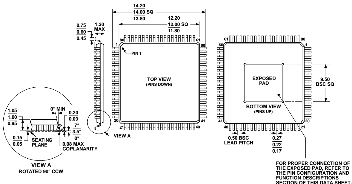
Figure 57. 80-Lead Thin Quad Flat Package, Exposed Pad [TQFP_EP]
