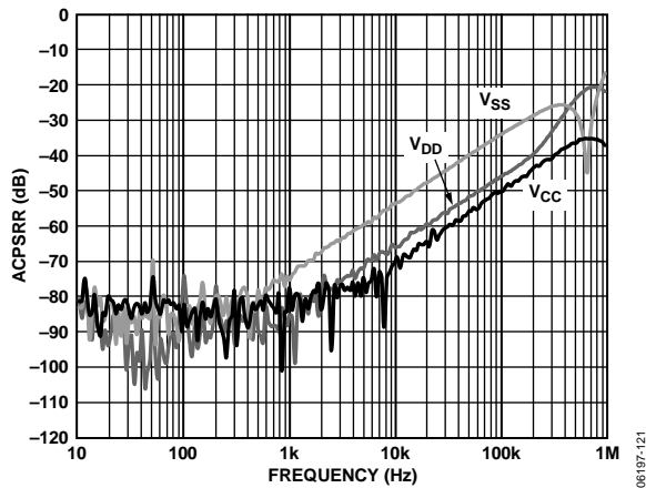
Figure 24. APCSR at MEASOUTx in Measure Current Mode vs. Frequency (MI Gain = 5, Measout Gain = 1)
