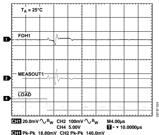
Figure 29. AC Crosstalk, FVMI Mode, PMU 1, Full-Scale Transition on One CPH DAC, MI Gain = 10, MEASOUTx Gain = 1, \pm 2 mA Range, C_{LOAD} = 200 pF
