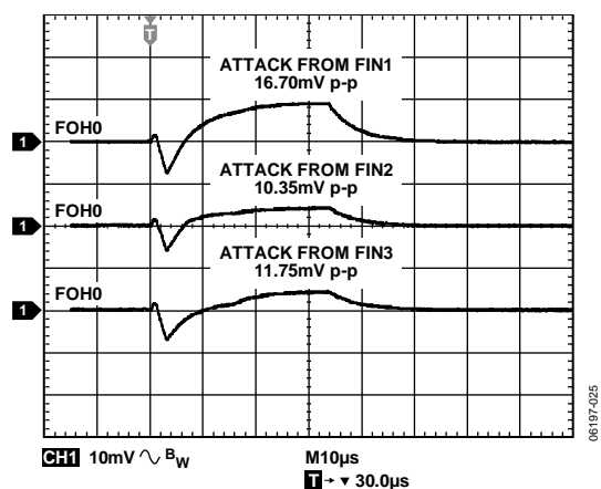
Figure 30. AC Crosstalk at FOH0 in FI Mode from FIN DAC of Each Other PMU (Full-Scale Transition), MI Gain = 10, MEASOUTx Gain = 1, \pm 2 mA Range, C_{LOAD} = 200 pF
