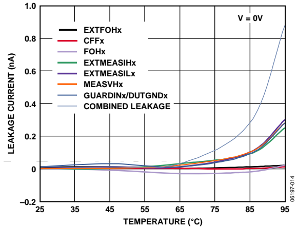
Figure 14. Leakage Current vs. Temperature (Stress Voltage = 0 V)
