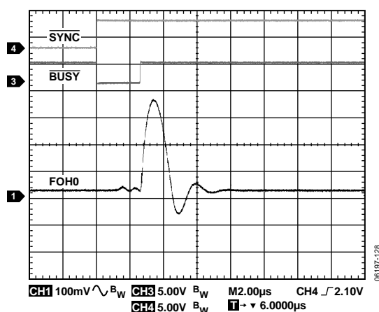
Figure 33. Range Change, PMU 0, \pm 5 \mu A to \pm 2 mA, C_{LOAD} = 1 nF, R_{LOAD} = 620 k \Omega , FV = 3 V
