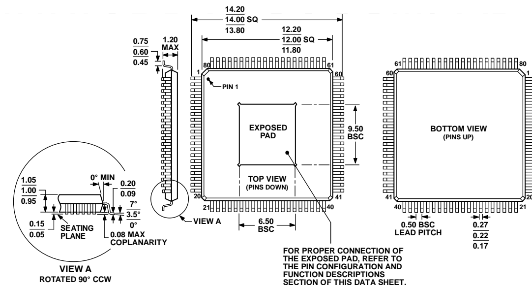
Figure 58. 80-Lead Thin Quad Flat Package, Exposed Pad [TQFP_EP]
