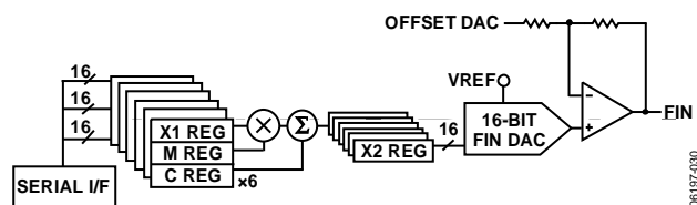
Figure 48. FIN DAC Registers
