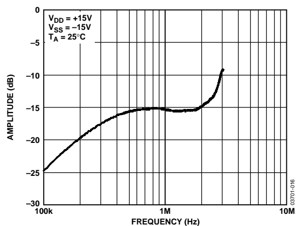
Figure 16. Force Amplifier AC PSRR, Mode 3, C_{COMP} = 100\text{pF}
