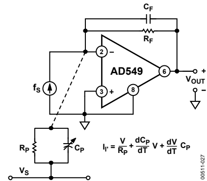
Figure 27. Sources of Parasitic Leakage Currents
