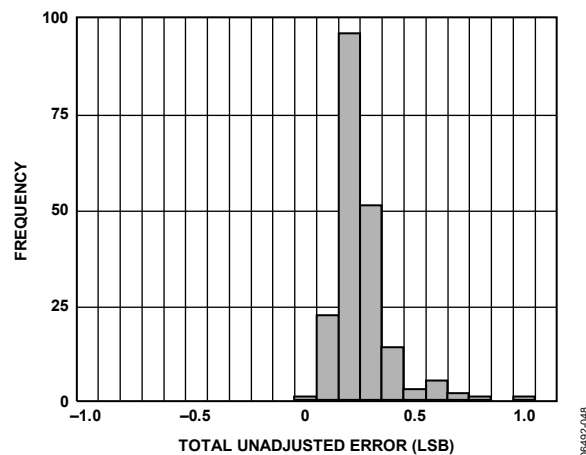
Figure 10. Total Unadjusted Error Histogram
