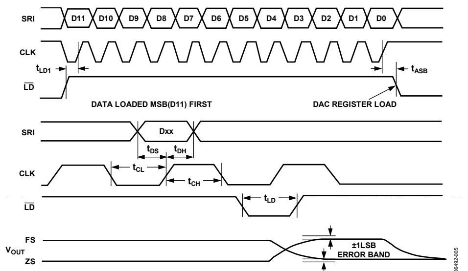
Figure 2. Timing Diagram
