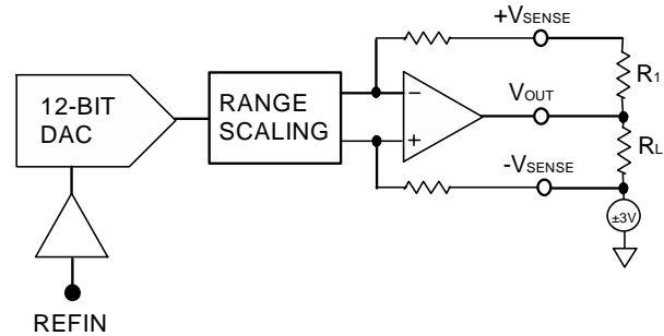
Figure 59. Voltage Output
