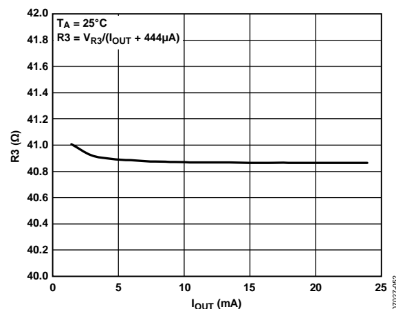
Figure 48. R3 Resistor Value vs. I_{OUT}
