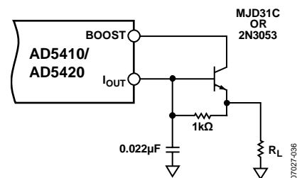
Figure 40. External Boost Configuration
