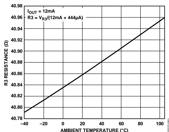
Figure 47. R3 Resistor Value vs. Temperature
