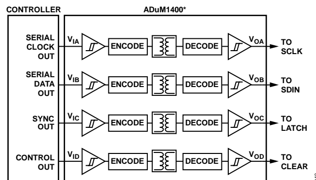
Figure 50. Isolated Interface
