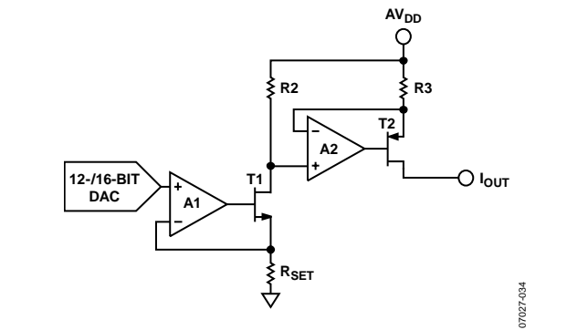
Figure 38. Voltage-to-Current Conversion Circuitry
