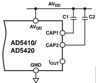
Figure 42. I OUT Filtering Capacitors
