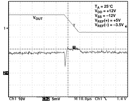
Figure 17. DAC-to-DAC Crosstalk
