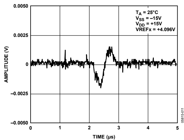
Figure 11. Digital Crosstalk
