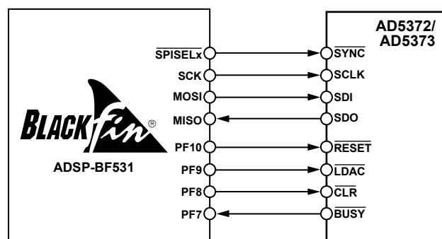
Figure 21. Interfacing to a Blackfin DSP
