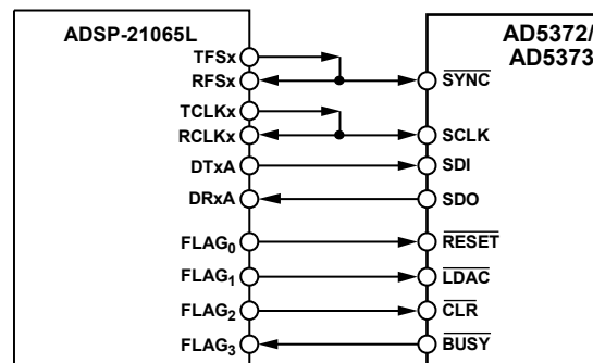
Figure 22. Interfacing to an ADSP-21065L DSP
