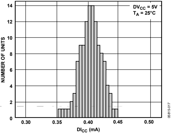
Figure 17. Typical D_{ICC} Distribution
