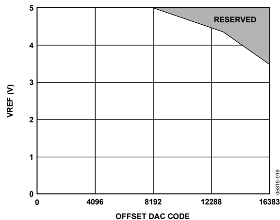
Figure 19. Offset DAC Code Range
