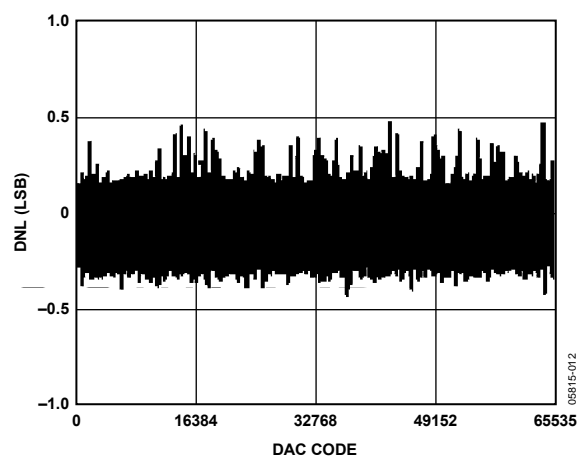
Figure 12. Typical AD5372 DNL Plot
