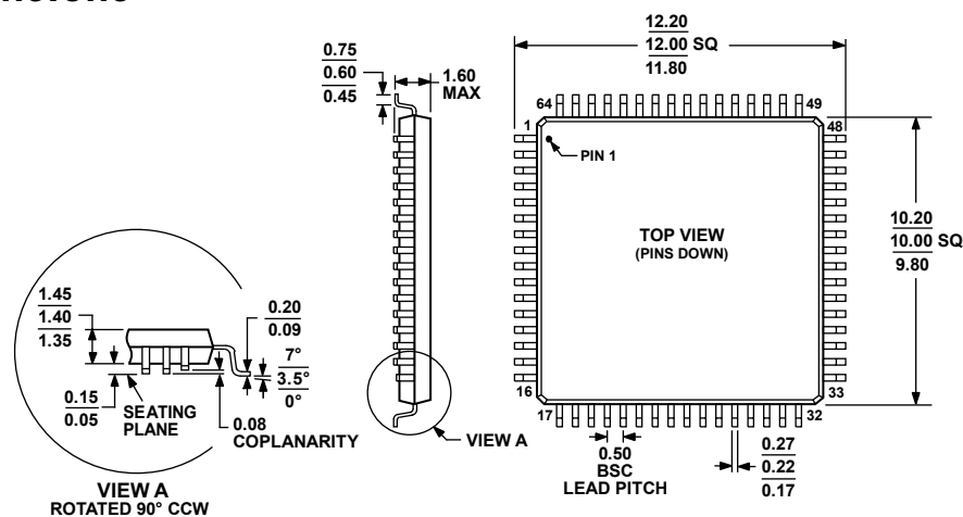
COMPLIANT TO JEDEC STANDARDS MS-026-BCD Figure 23. 64-Lead Low Profile Quad Flat Package [LQFP] (ST-64-2) Dimensions shown in millimeters
