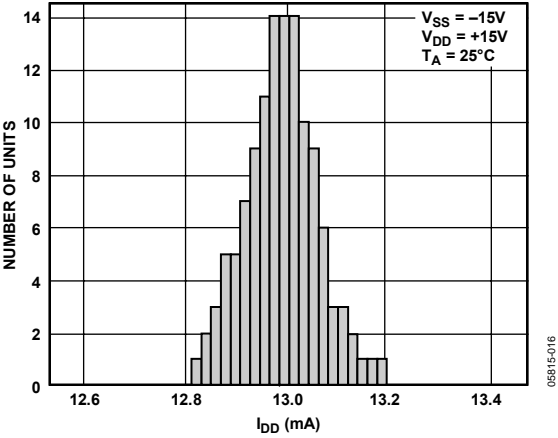
Figure 16. Typical I_{BD} Distribution
