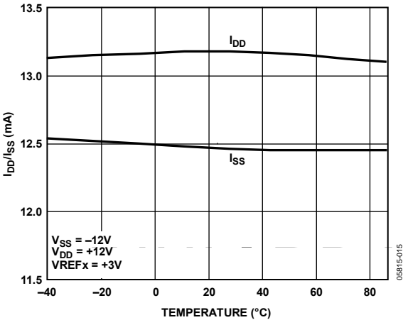
Figure 15. I_{BD}/I_{SS} vs. Temperature
