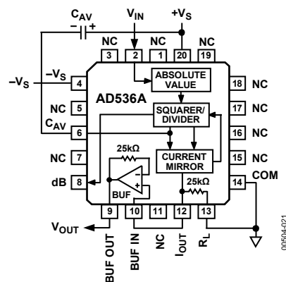
Figure 8. 20-Terminal Standard RMS Connection
