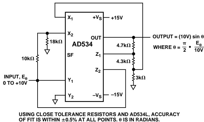
Figure 10. Sine-Function Generator
