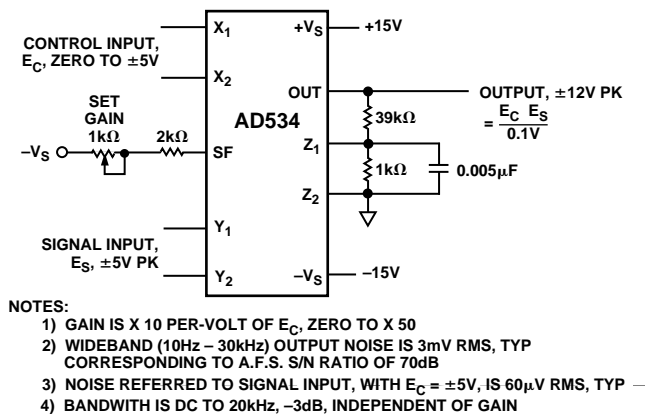
Figure 9. Voltage-Controlled Amplifier
