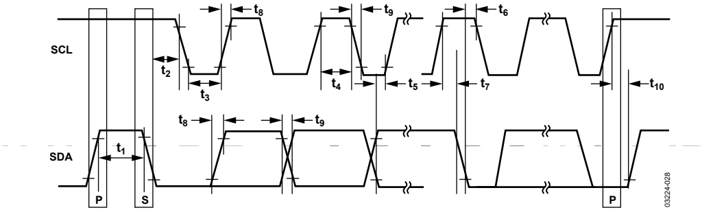
Figure 29. Interface Timing Diagram
