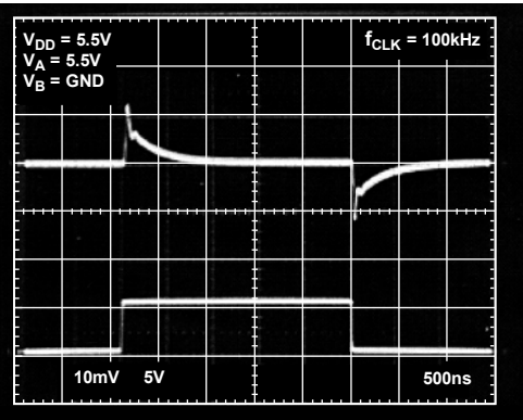
Figure 23. Digital Feedthrough
