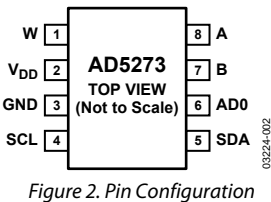
Figure 2. Pin Configuration
