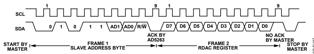
Figure 44. Reading Data from a Previously Selected RDAC Register in Write Mode
