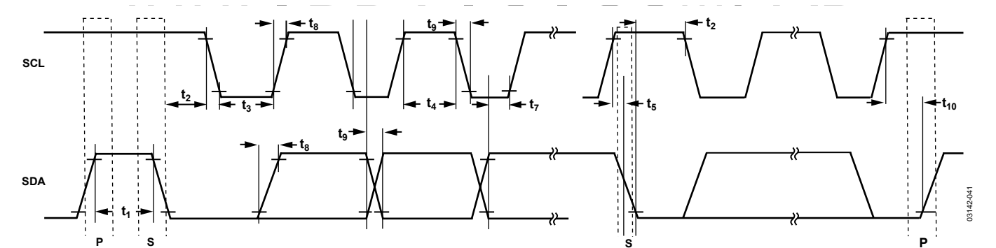
Figure 42. Detailed I 2 C Timing Diagram
