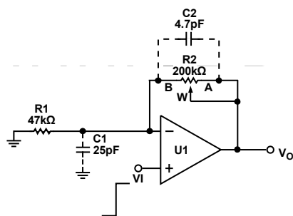
Figure 58. Typical Noninverting Gain Amplifier
