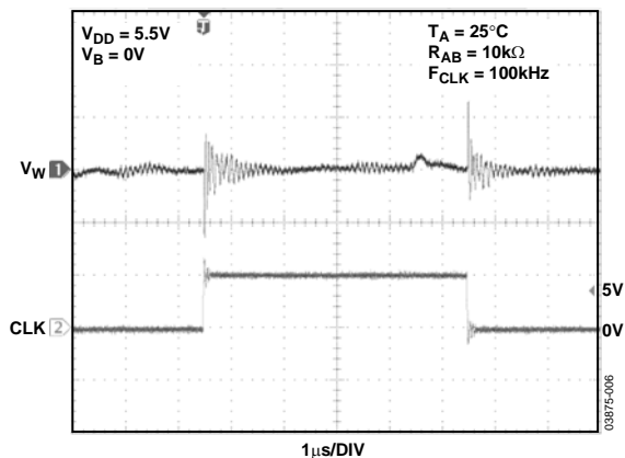
Figure 18. Digital Feedthrough
