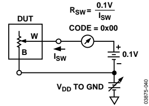
Figure 24. Test Circuit for Incremental On Resistance
