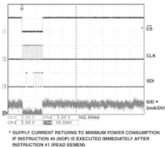
TPC 9. I_{DD} vs. Time Read Mode
