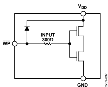
Figure 38. Equivalent \overline{\text{WP}} Input Protection
