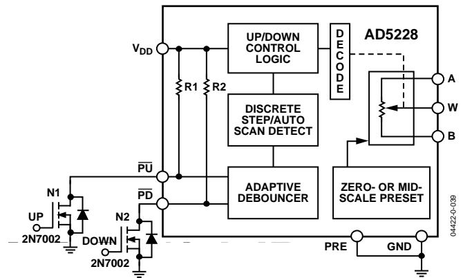
Figure 38. Digital Control with External MOSFETs
