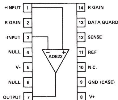
14-Pin DIP
