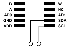
Figure 44. Recommended AD5170 PCB Layout
