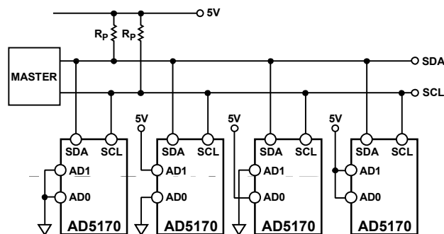
Figure 47. Multiple AD5170s on One I 2 C Bus
