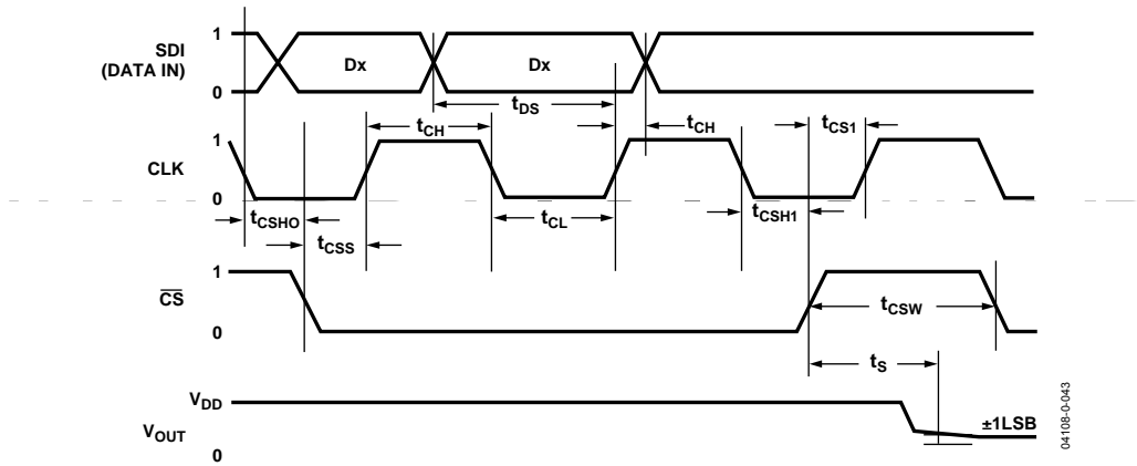
Figure 43. SPI Interface Detailed Timing Diagram ( V_A = 5\text{ V} , V_B = 0\text{ V} , V_W = V_{OUT} )
