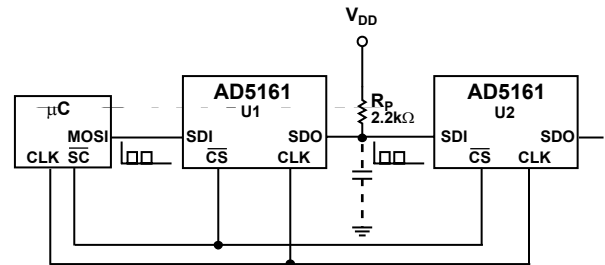
Figure 42. Daisy-Chain Configuration
