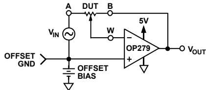
Figure 31. Test Circuit for Inverting Gain
