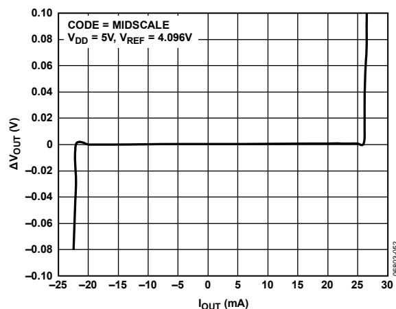
Figure 41. Typical Current Limiting Plot
