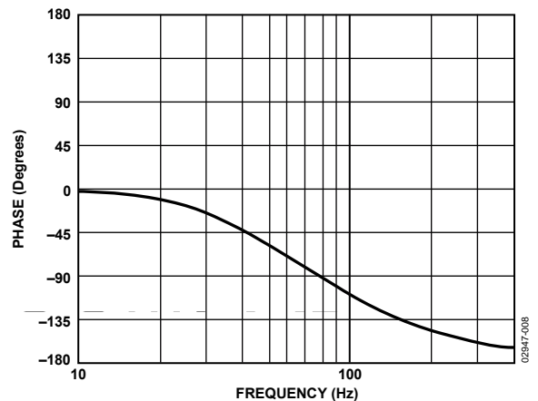
Figure 8. Phase Plot
