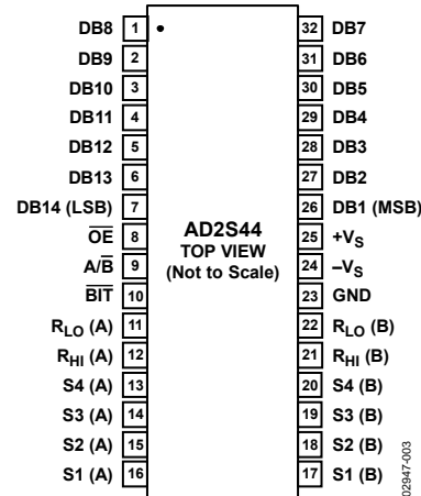
Figure 2. Pin Configuration
