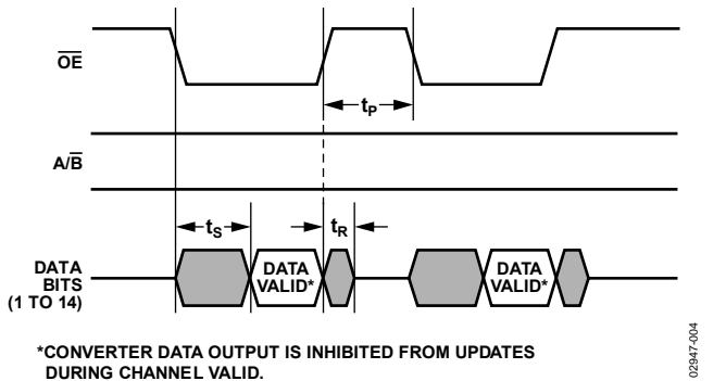
Figure 5. Alternative Reading of Each Channel
