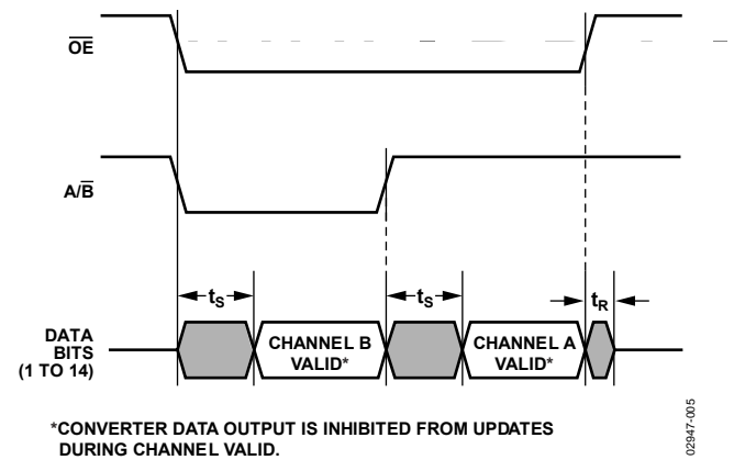
Figure 4. Repetitive Reading of One Channel
