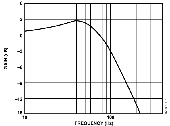
Figure 7. Gain Plot
