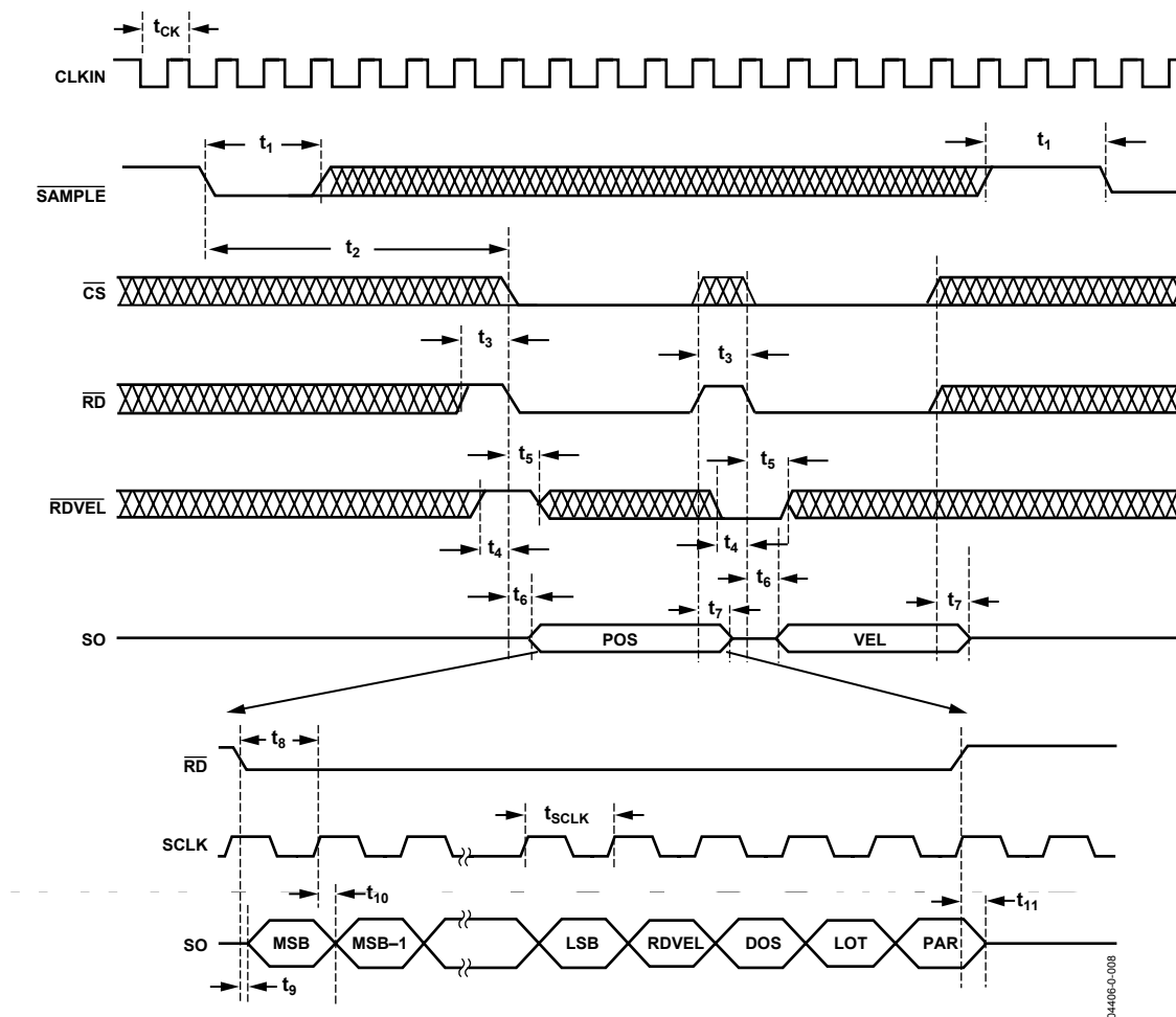
Figure 8. Serial Port Read Timing
