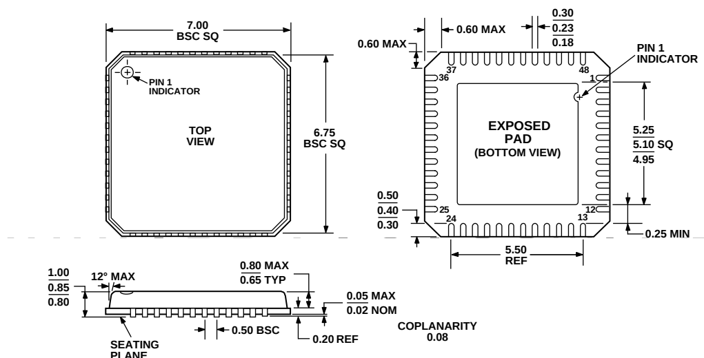
Figure 6. 48-Lead Lead Frame Chip Scale Package [LFCSP_VQ] 7 mm × 7 mm Body, Very Thin Quad (CP-48-1)
