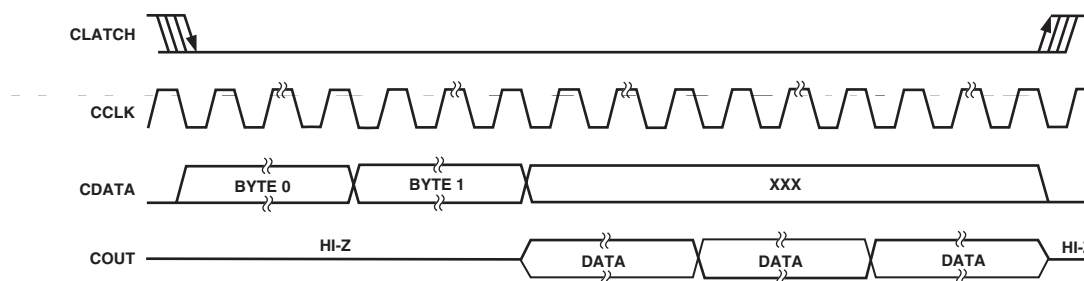
Figure 17. Sample of SPI READ Format (Single-Read Mode)
