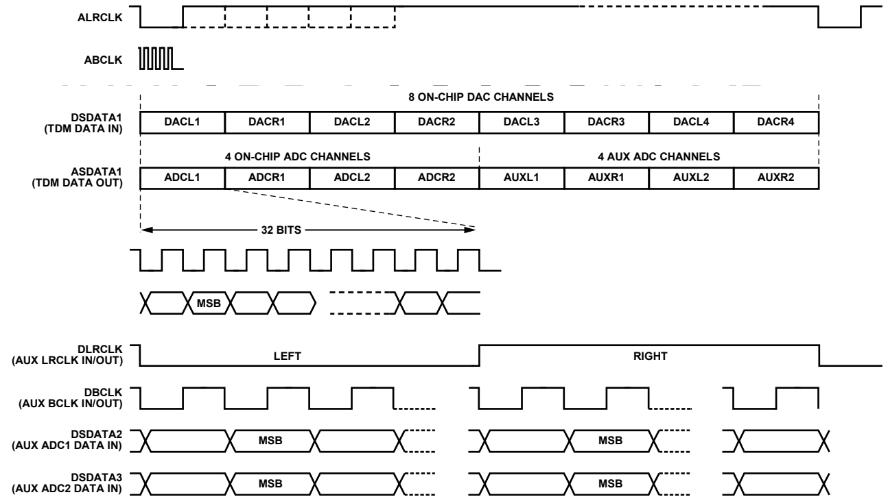
Figure 19. TDM/AUX Mode 8-Channel ADC Configuration
