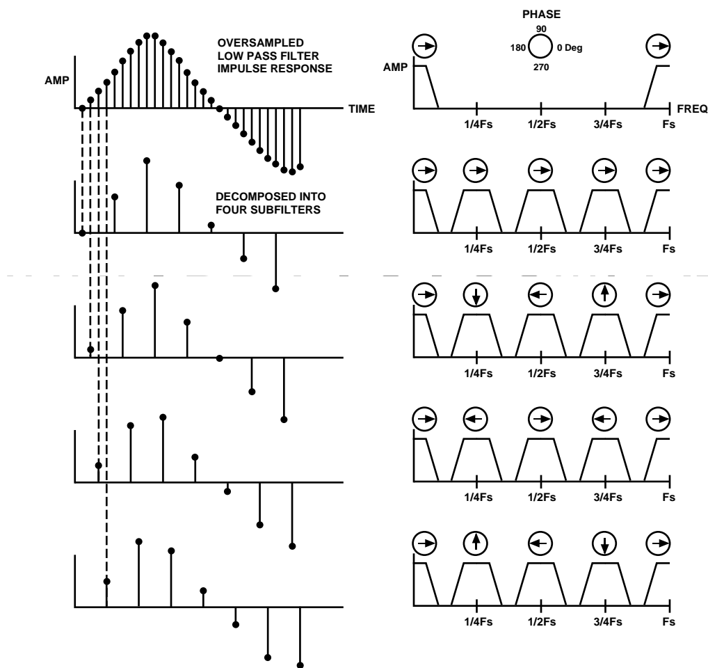
Figure 2. Four Polyphase Subfilters in the Time and Frequency Domains
