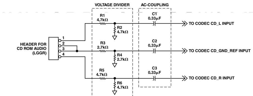
Figure 12. Typical CD-ROM Audio Connections
