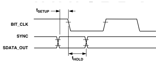
Figure 4. Data Setup and Hold
