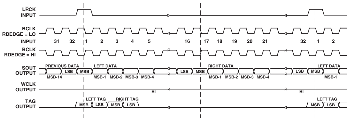
Figure 15. Serial Data Output Timing: Slave Mode, Left-Justified with No MSB Delay, 32-Bit Frame Mode, \overline{S\overline{M}} = \text{HI} , \overline{R\overline{LJUST}} = \text{LO} , \overline{MSBDLY} = \text{HI}
