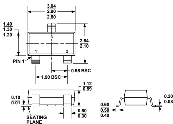
Figure 27. 3-Lead Small Outline Transistor Package [SOT-23-3] (RT-3)
