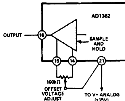
Figure 3. AD1362 Offset Voltage Adjustment
