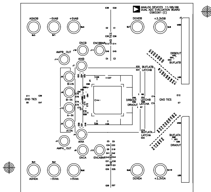
Figure 24. Top Silk
