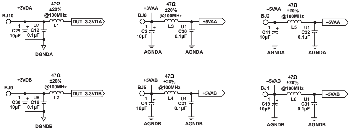
Figure 21. Evaluation Board
