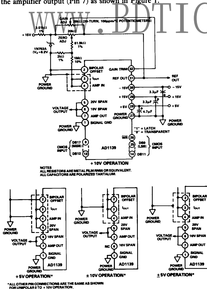
Figure 1. Output Voltage and Trim Configuration
