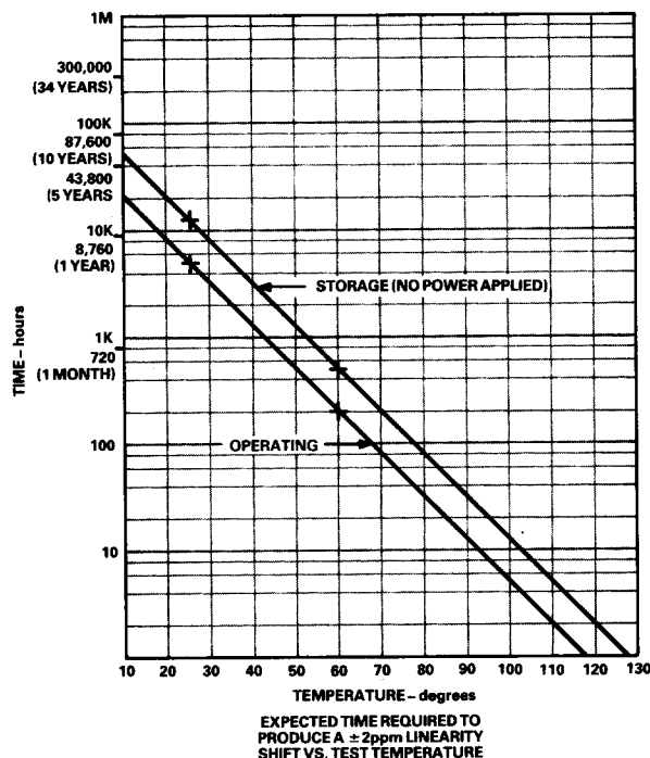
Figure 7. Nonlinearity vs. Time/Temperature
