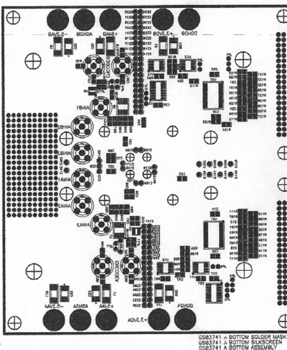
Figure 34. Bottom Assembly
