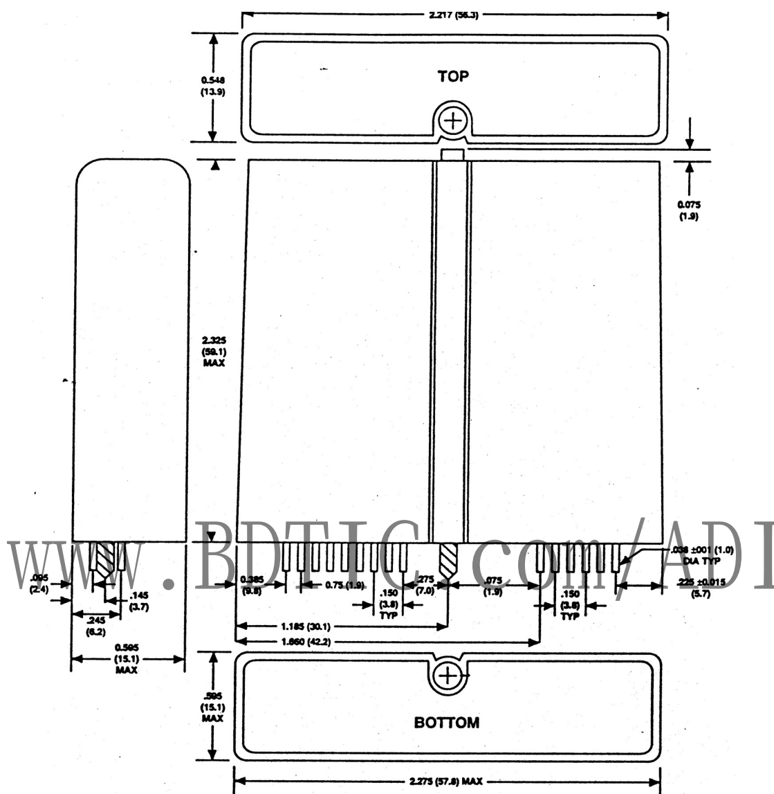
Figure 5. Outline Dimensions
