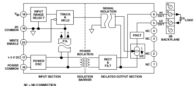
Figure 1. 5B39 Functional Block Diagram
