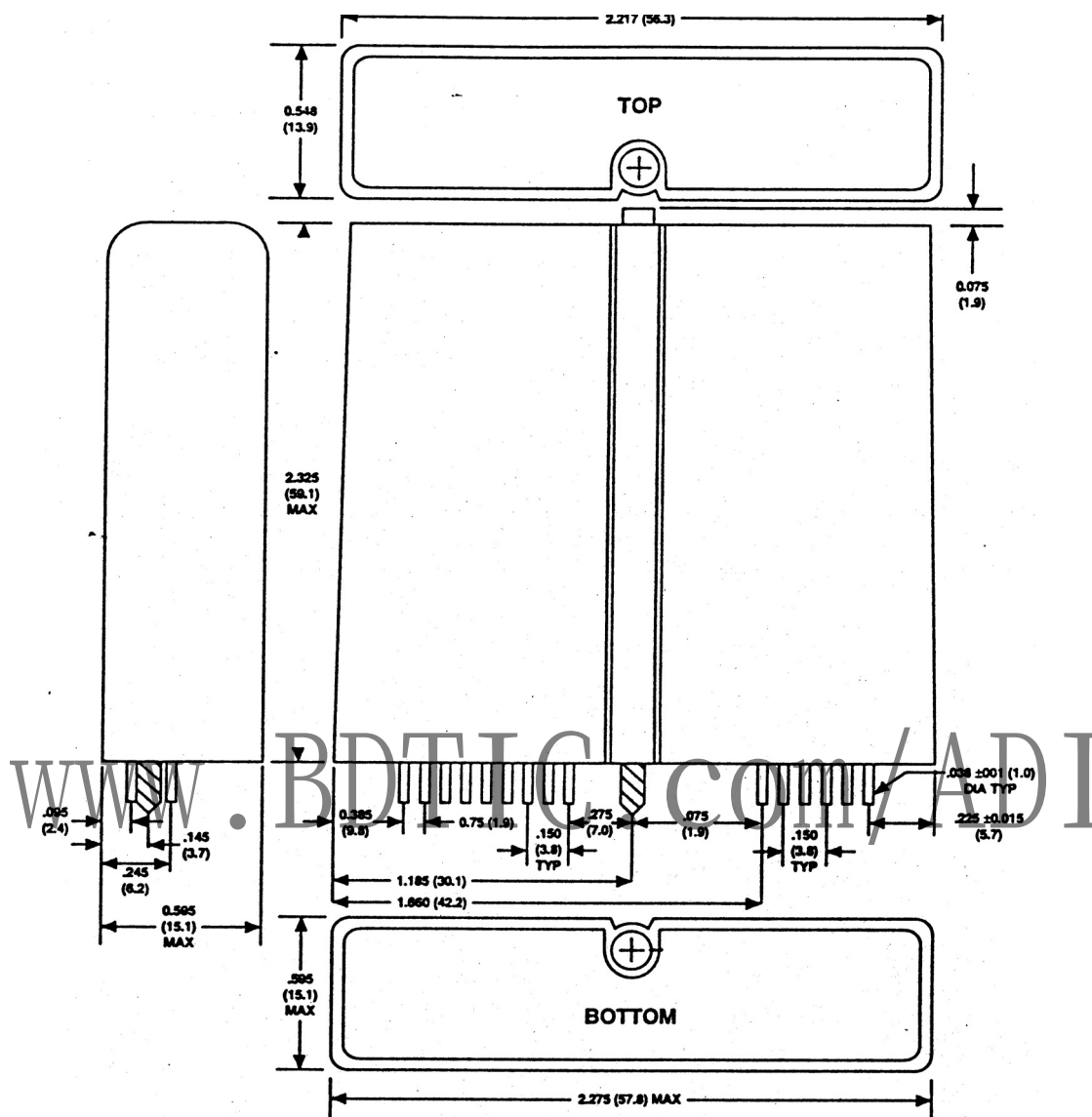
Figure 5. Outline Dimensions
