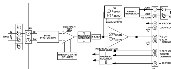
Figure 1. 3B32 Functional Block Diagram
