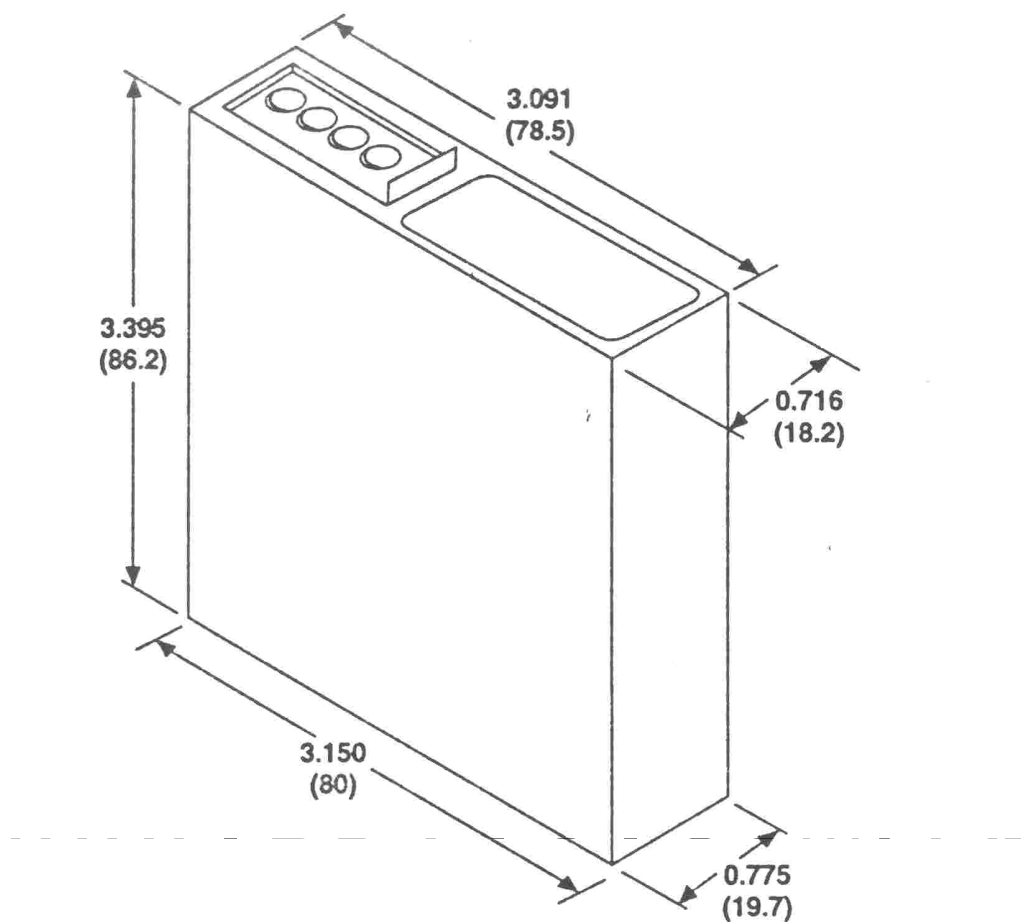
Figure 5. Outline Dimensions
