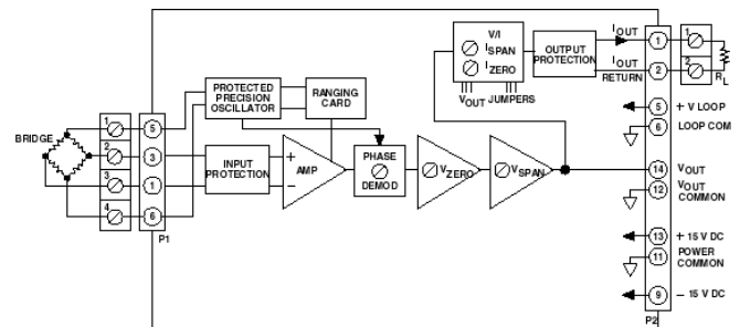
Figure 1. 3B20 Functional Block Diagram
